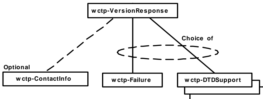
Figure 6 – wctp-VersionResponse Entity
